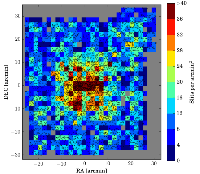
Figure 2. Two dimensional spatial density of VIMOS slits. Slits are shown as small black crosses, whereas the colours represent total counts in boxes of 2 \times 2 arcmin 2 . Axes express the distance in arcmin from NGC 1399. More slits were placed towards the center of the cluster, where the target density is higher. North is toward the top, East to the left.
