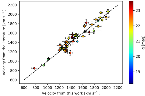
Figure 6. Comparison with literature studies. The radial velocity of literature objects is averaged among literature studies as discussed in the text. The 1-to-1 line is shown as a dashed line.
