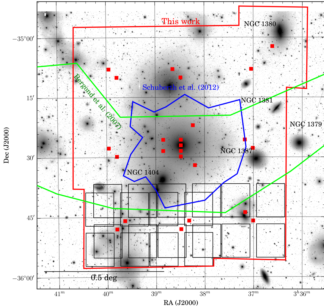
Figure 1. Layout of the observations. The background image is a mosaic of several VST/OmegaCAM pointings in the g -band. The central galaxy is NGC 1399. Additional Fornax galaxies are also labeled. The red boxes mark the centers of all 25 VIMOS pointings. The footprints of some VIMOS masks are shown on the bottom for illustrative purposes. Note how the VIMOS masks are dithered to maximize spatial coverage. The region covered by all 25 VIMOS is outlined in red, whereas the regions covered by literature studies are shown in green (Bergond et al. 2007) and blue (Schuberth et al. 2010).
