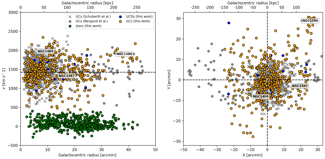
Figure 7. Left: Phase-space velocity diagram. The figure shows the measured systemic velocity of the Fornax objects presented in this paper (orange points), GCs from Schuberth et al. (2010) (grey crosses), GCs from Bergond et al. (2007) (grey points) and Galactic stars measured in this paper (green points). The systemic velocity of NGC 1399 is marked with a dashed line at v = 1425 km s -1 . The systemic velocity and galactocentric distance of giant Fornax galaxies (namely NGC 1404, NGC 1387, NGC 1380) are marked with the correspondent galaxy name. The distance is expressed in arcminutes from the centre of NGC 1399. Physical distances in kpc are also shown on the top panel. Right: Position diagram, with North to the top and East to the left. The plot shows the spatial distribution of the objects from the left panel (except for Galactic stars for clarity). Note how the GCs from our paper complement the GC catalogues of Schuberth et al. (2010) and Bergond et al. (2007).
