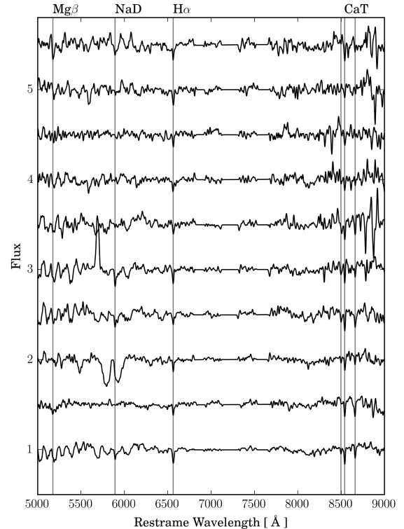
Figure 4. A sample of GC spectra suitably normalised. Shown are continuum-normalized redshift-corrected spectra for GCs with increasing S/N per resolution element (from top to the bottom). The spectrum at the top has S/N = 15 , the one at the bottom S/N = 50 . The main atomic lines are labelled on the top. Features such as the strong absorption in the spectrum at Flux = 2 and the emission in the spectrum at Flux = 3 are instrumental artifacts and not physical features of the GC. The flat horizontal lines between 7000–8000 Å mark regions with masked skylines (see text).
