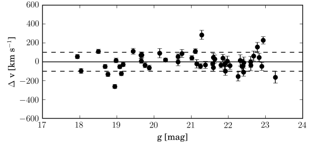
Figure 5. Internal velocity comparison. The figure shows the velocity difference \Delta v between GCs with two independent velocity measurements. The solid and dashed line represent the reference \Delta v = 0 \text{ km s}^{-1} and \Delta v = \pm 100 \text{ km s}^{-1} , respectively.
