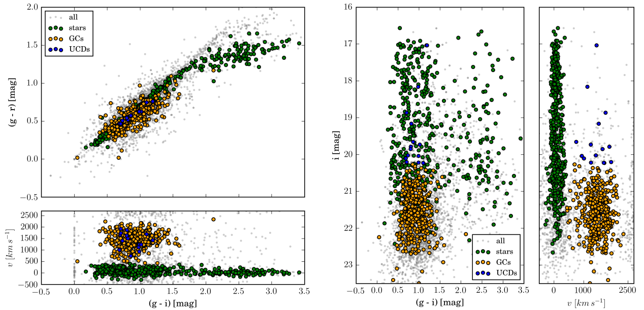
Figure 8. Colour–colour and colour–magnitude diagram. The figure shows the distribution of the labelled objects in a (g-i) vs. (g-r) space (left panel) and (g-i) vs i space (right panel). Each diagram includes also a radial velocity v axis to show the separation of GCs/UCDs from stars and galaxies. The objects labelled as ‘all’ represent all 4340 sources observed with VIMOS.
