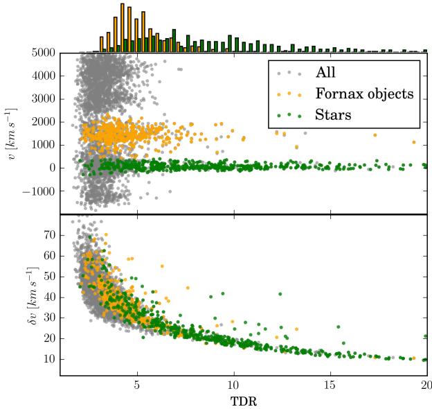
Figure 3. Results from iraff/xcor for \sim 4200 spectra. The x-axis represents the Tonry & Davies R parameter (TDR) which is a proxy for the goodness of the cross-correlation between the scientific and the template spectra. Smaller TDR corresponds to larger velocity uncertainties \delta v (bottom panel) and therefore to a poorer spectral fit. The measured radial velocity v is shown on the y-axis of the top panel. The sequence of objects at v \approx 0 \text{ km s}^{-1} are Galactic stars, whereas the cluster at v \approx 1700 \text{ km s}^{-1} are sources in the Fornax cluster. The histogram on the top shows raw counts for stars and Fornax objects, respectively.
